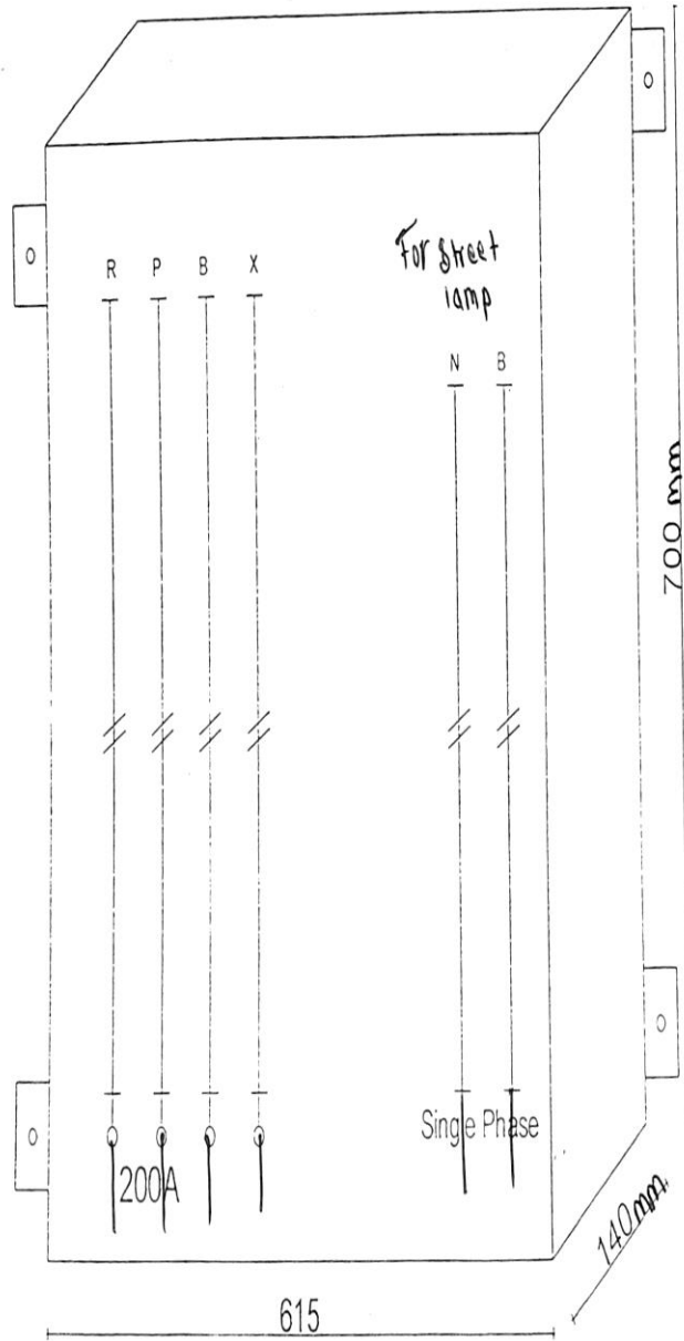
Copper Busbar Junction (Panel cabinet) Board-1 set
